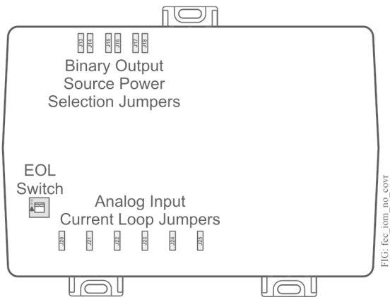
Figure 10: FAC26 with cover removed showing EOL switch and jumper positions
